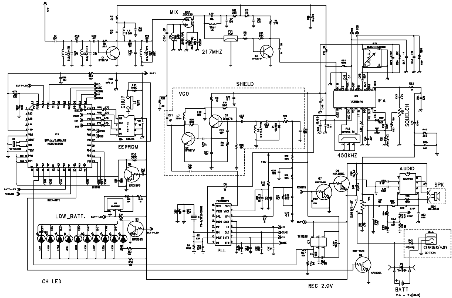
rx schmetic diagrams
